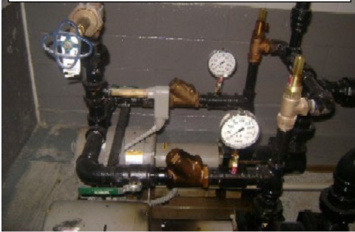
PUMP CONNECTED TO PIPING WITH THE PRESSURE GAUGE AND CONTROL VALVES
