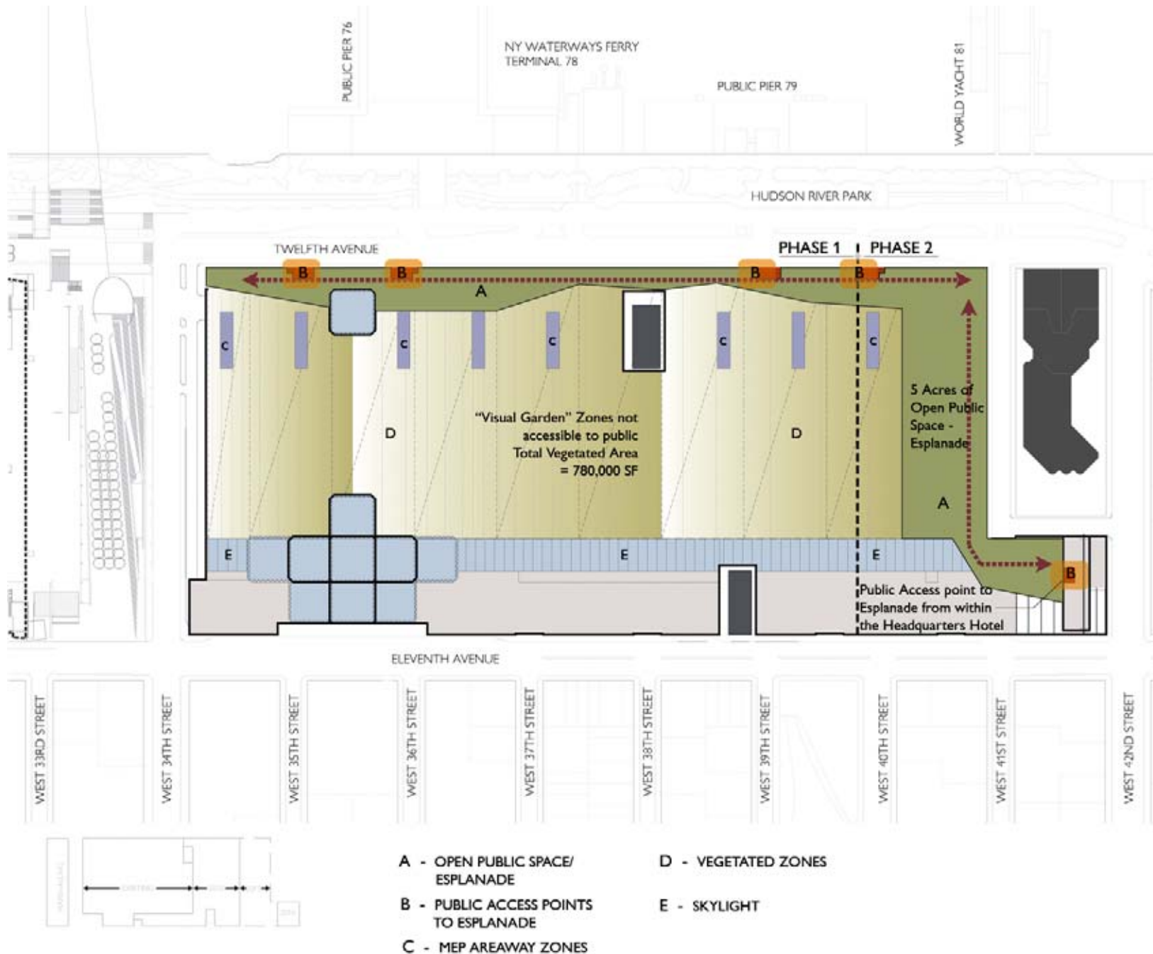
Convention Center: Rooftop Open Space Figure 7-6
