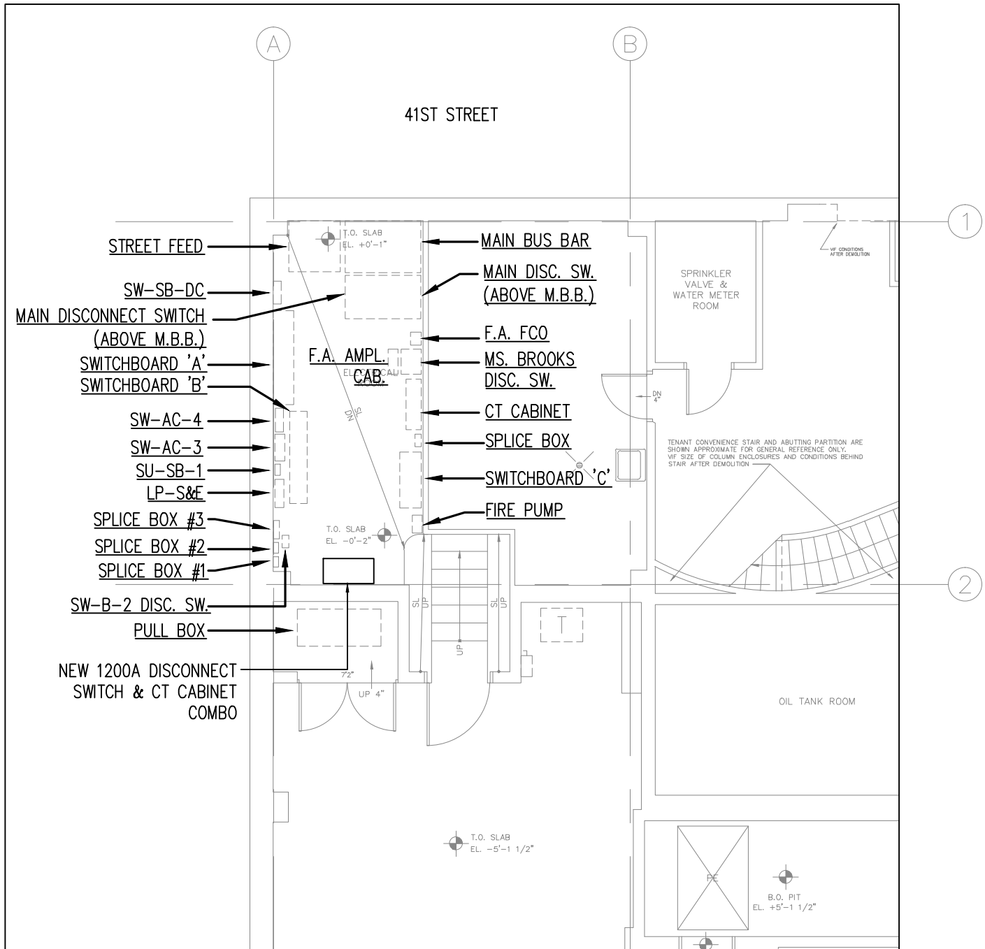
① ELECTRICAL CELLAR EXISTING POWER PART PLAN SCALE: 1/8" = 1'-0"
