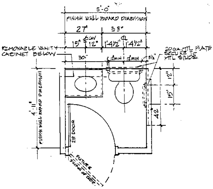
POWDER RM. PLAN WITH 27" REMOVABLE VANITY CABINET 'B5b' SCALE 1/2" = 1'-0"
