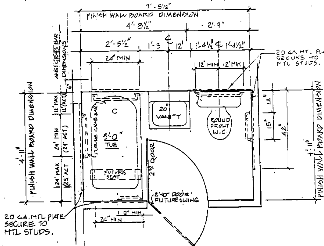
BATHROOM PLAN w/24" REMOVABLE VANITY CABINET 'B' 1/2" = 1'-0"
