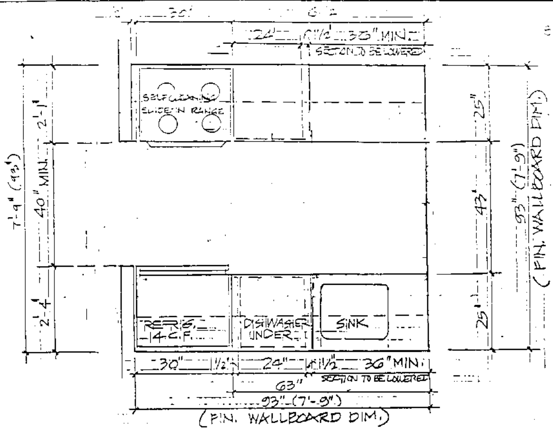
KITCHEN (GALLEY TYPE) 'K3a'
