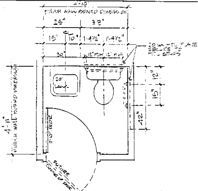
POWDER RM. PLAN WITH 20" LAVATORY 'B5a' SCALE 1/2" = 1'-0"
