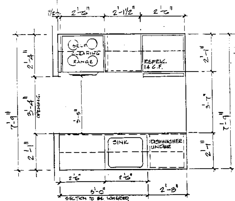
LAYOUT K2b KITCHEN (GALLEY TYPE) SCALE - 1/2" = 1'-0"
