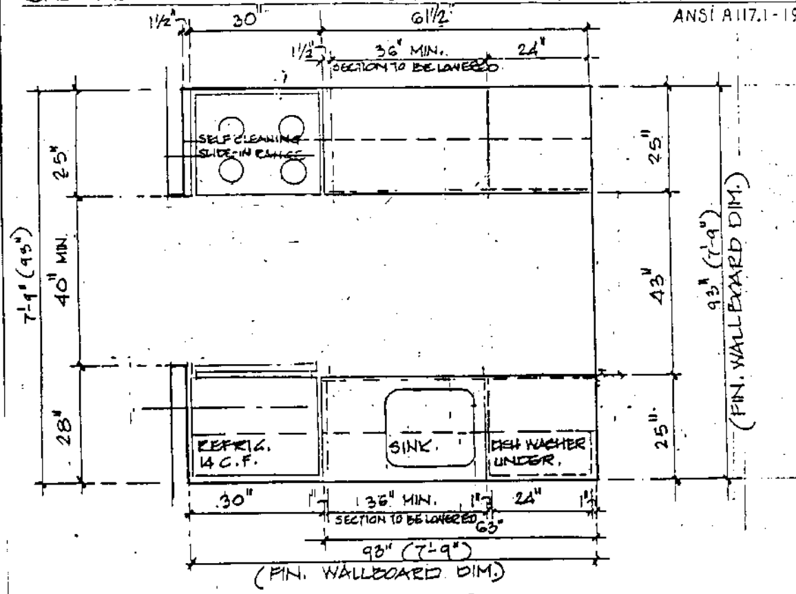
KITCHEN (GALLEY TYPE) 'K3b'
