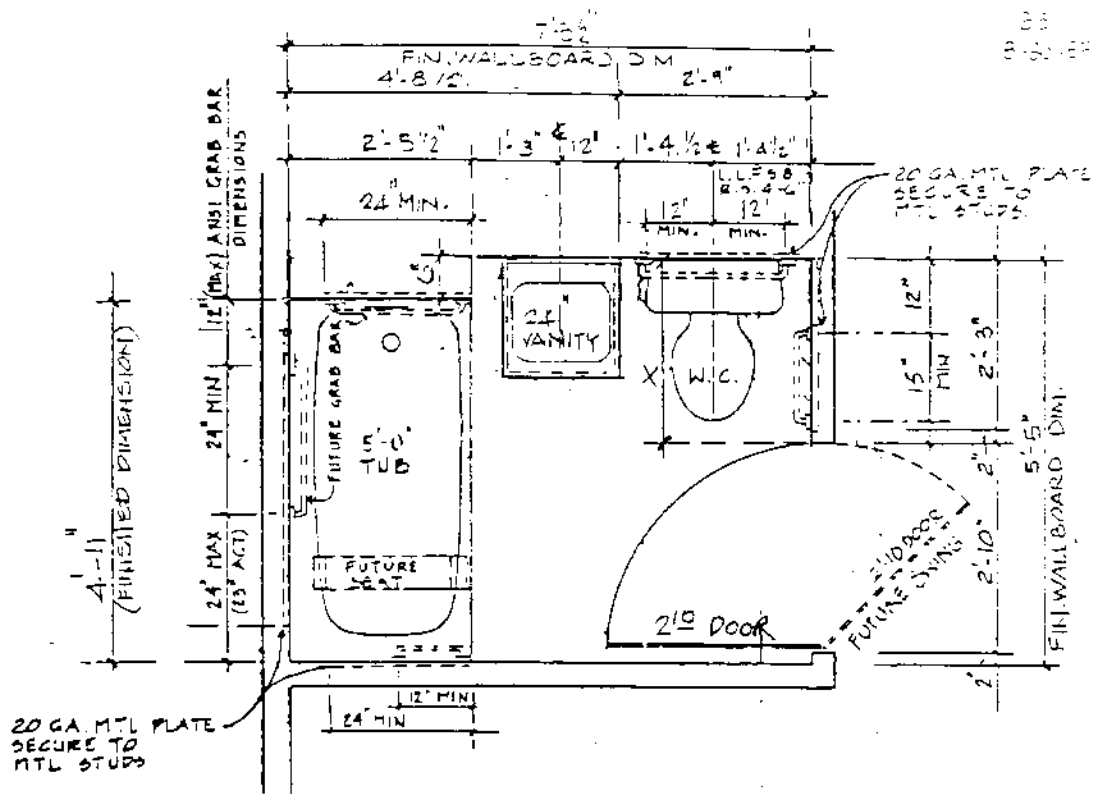
BATHROOM PLAN WITH 24" REMOVABLE VANITY CABINET.
