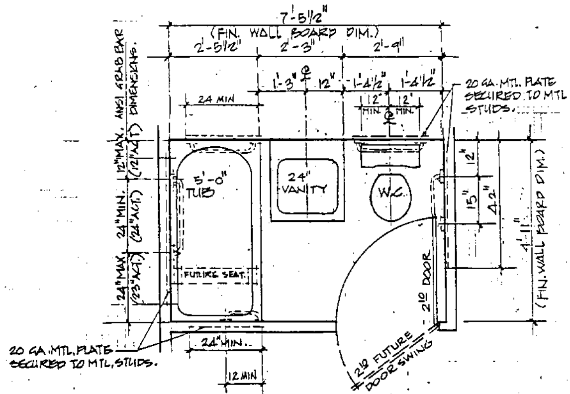
BATHROOM TYPE WITH 24" REMOVABLE VANITY CABINET B2b
