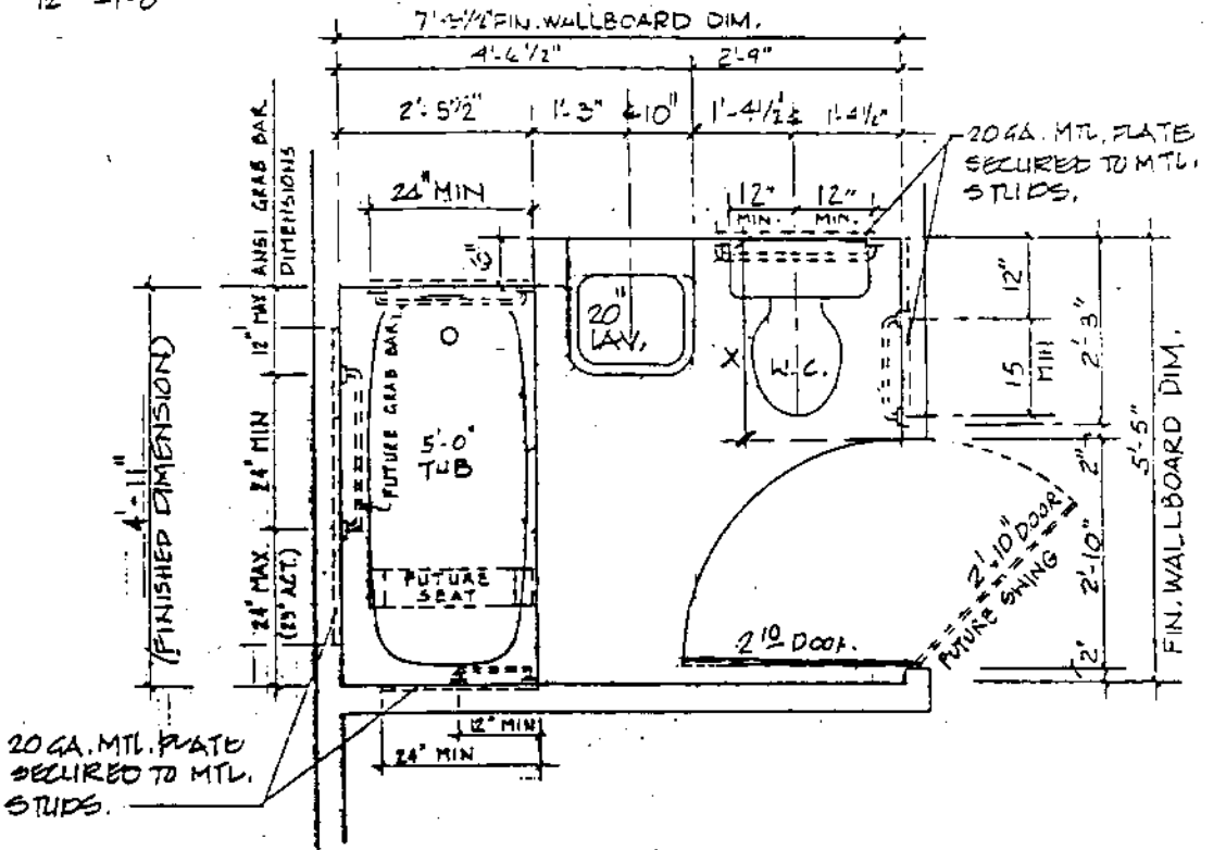
BATHROOM PLAN W/20" LAVATORY
