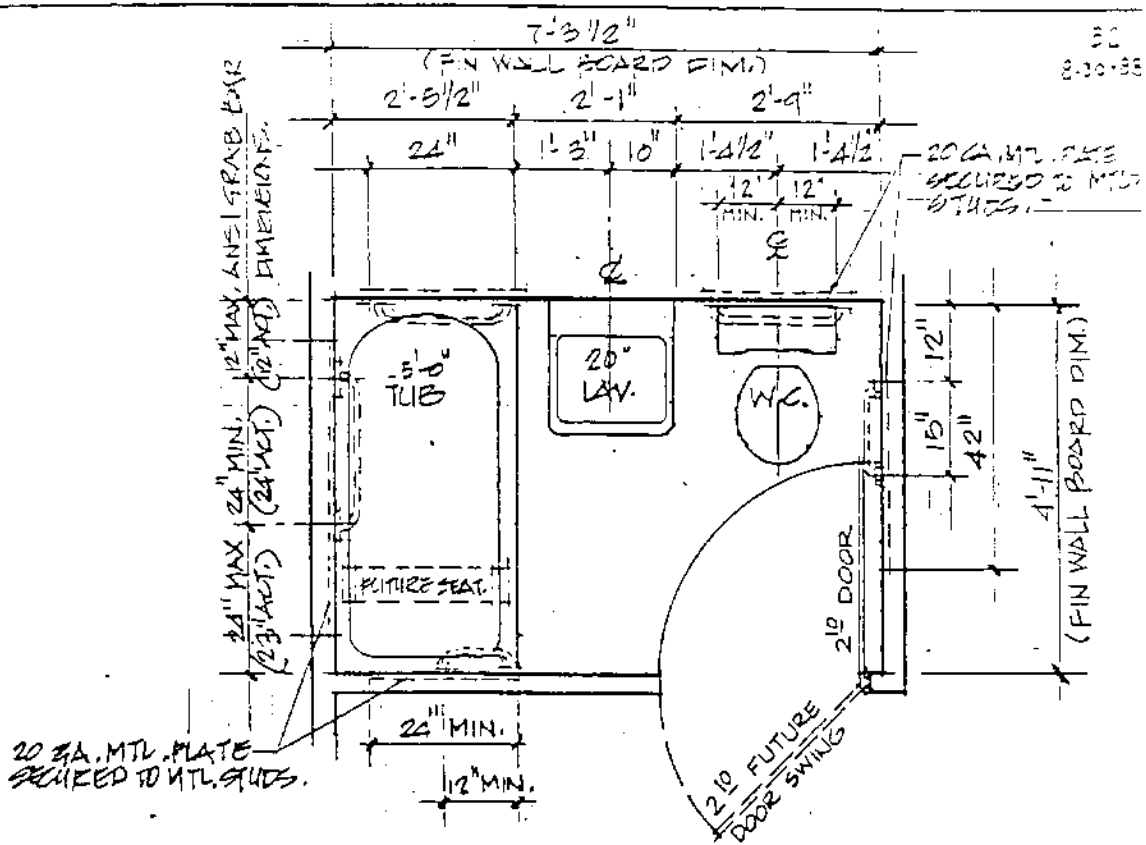
BATHROOM TYPE WITH 20" LAVATORY B2a
