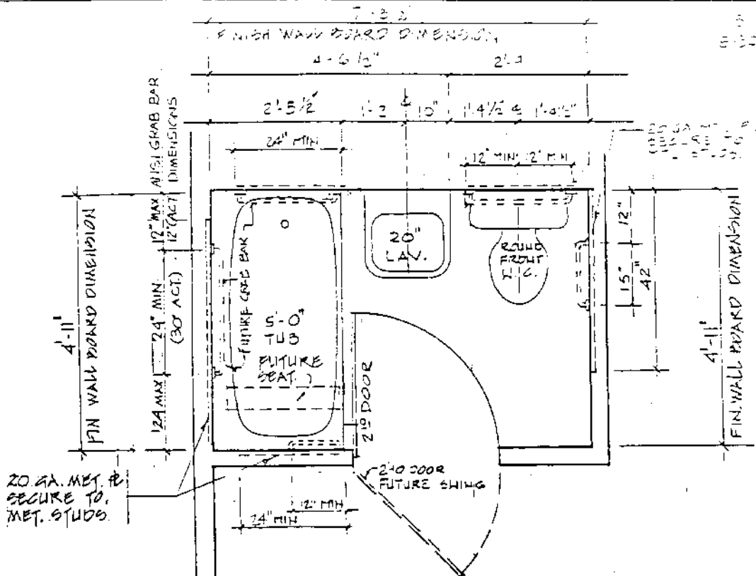
BATHROOM PLAN w/20" LAVATORY 'B1a' SCALE: 1/2" = 1'-0"
