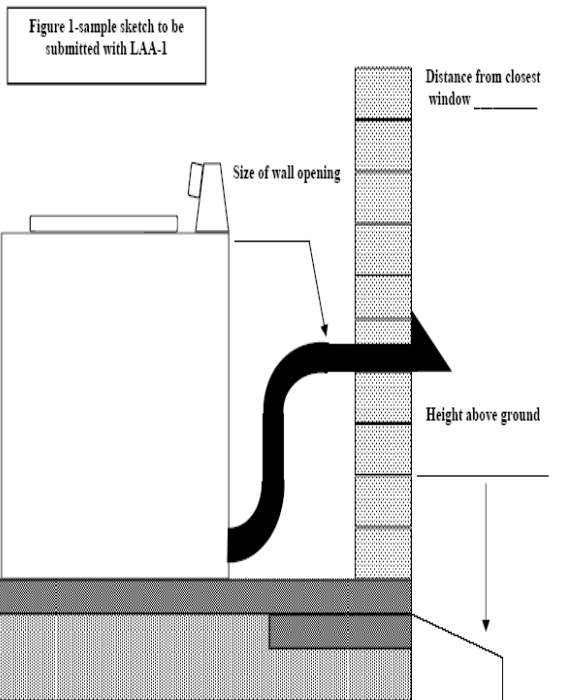
Domestic Gas Dryer Installation
