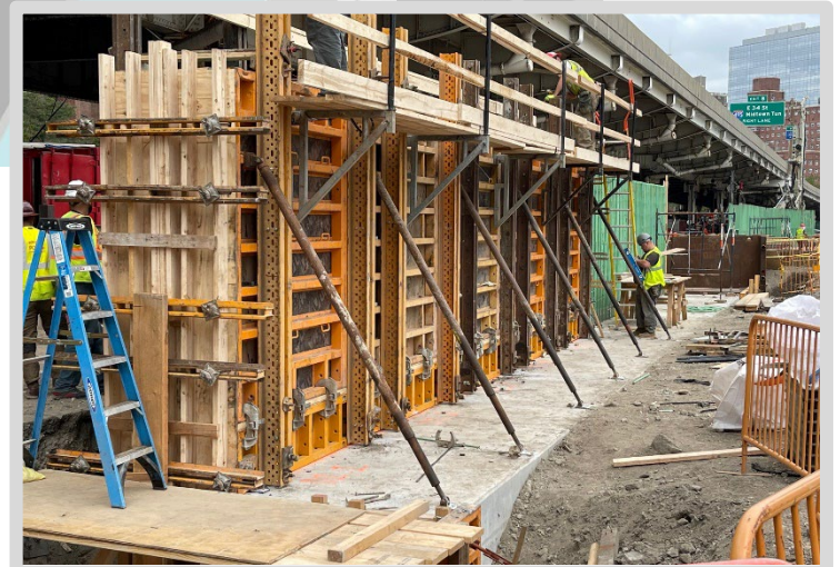
Operation 1: Flood wall form work.
