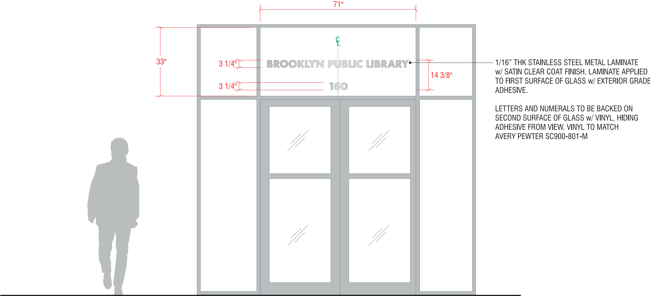
FRONT ELEVATION - TYP.
