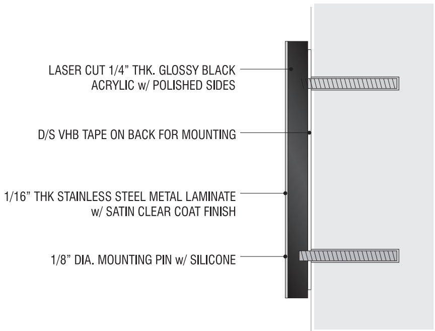
SECTION VIEW
