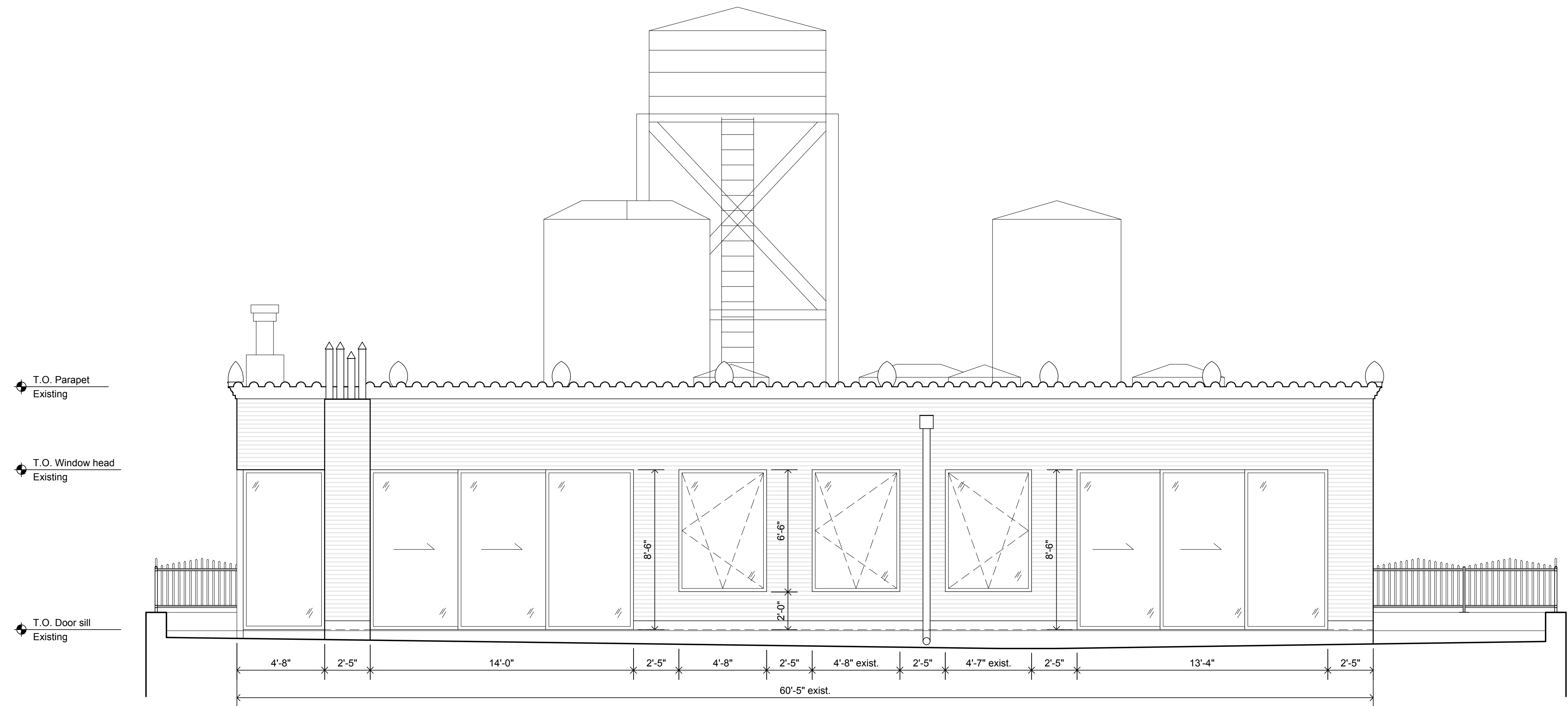
2 East Elevation Proposed 1/4"=1'-0"
