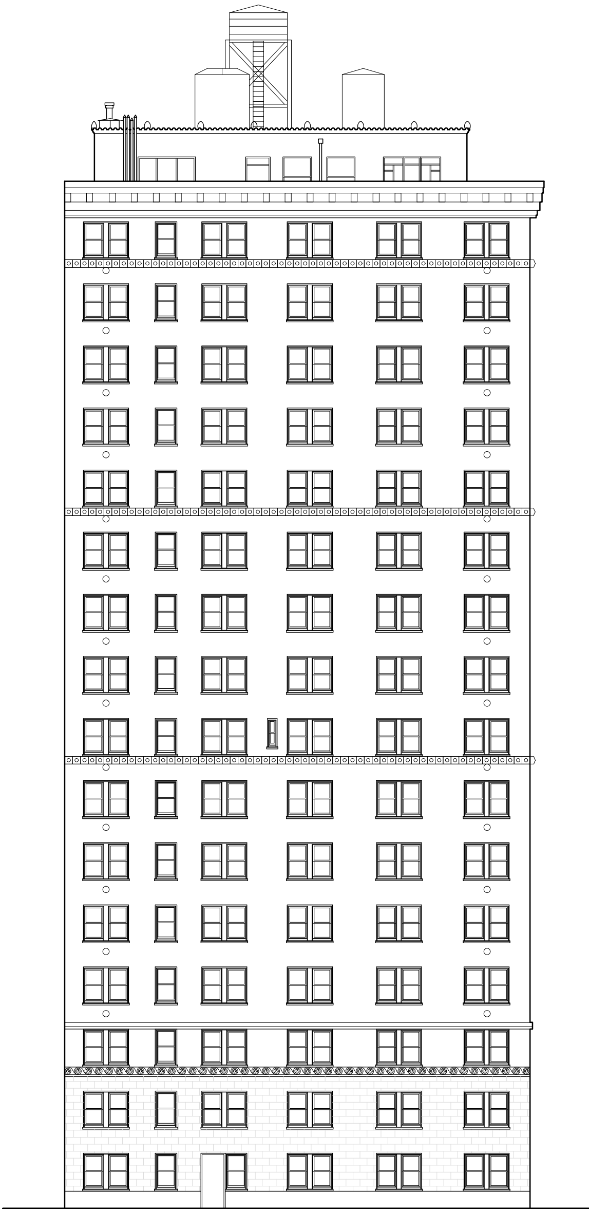
1 East Elevation Existing 1/16"=1'-0"
