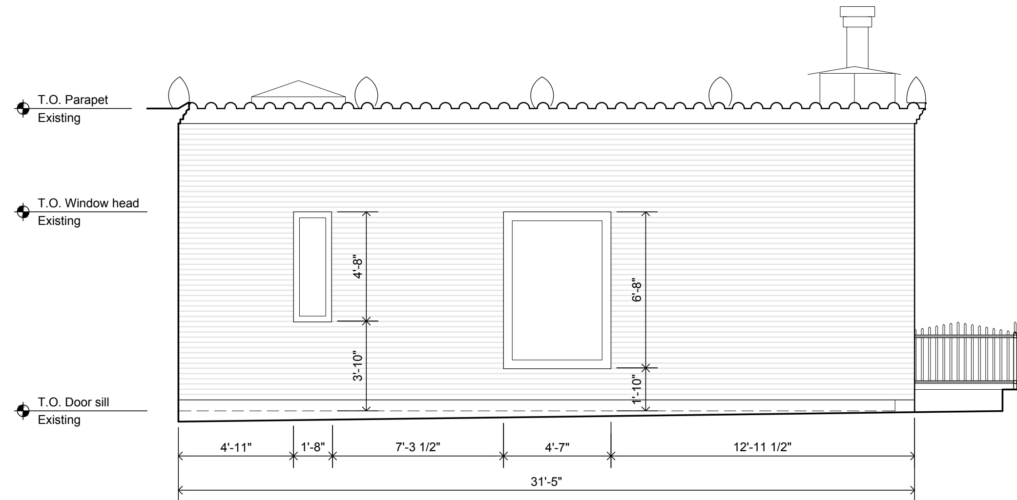
3 West Elevation Existing 1/4"=1'-0"
