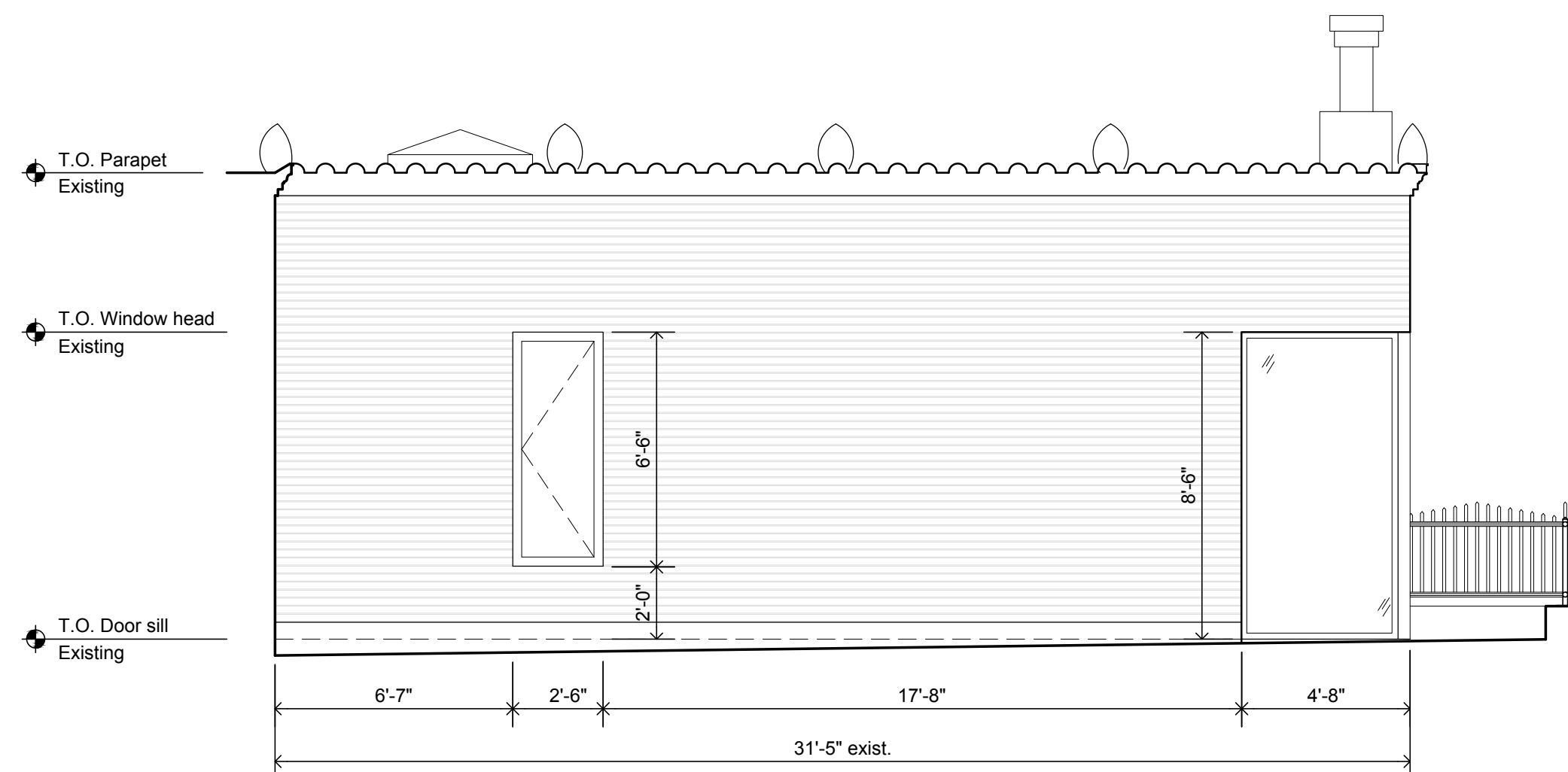
4 West Elevation Proposed 1/4"=1'-0"
