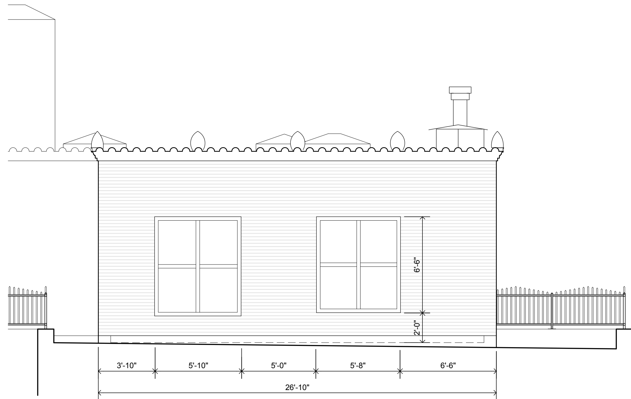
1 South Elevation Existing 1/4"=1'-0"
