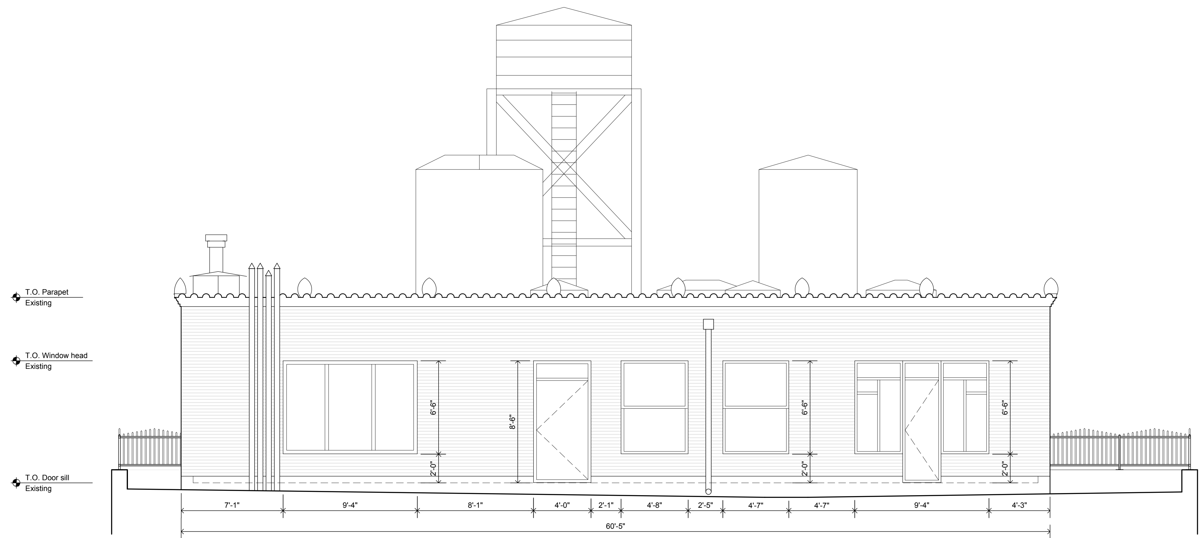
1 East Elevation Existing 1/4"=1'-0"
