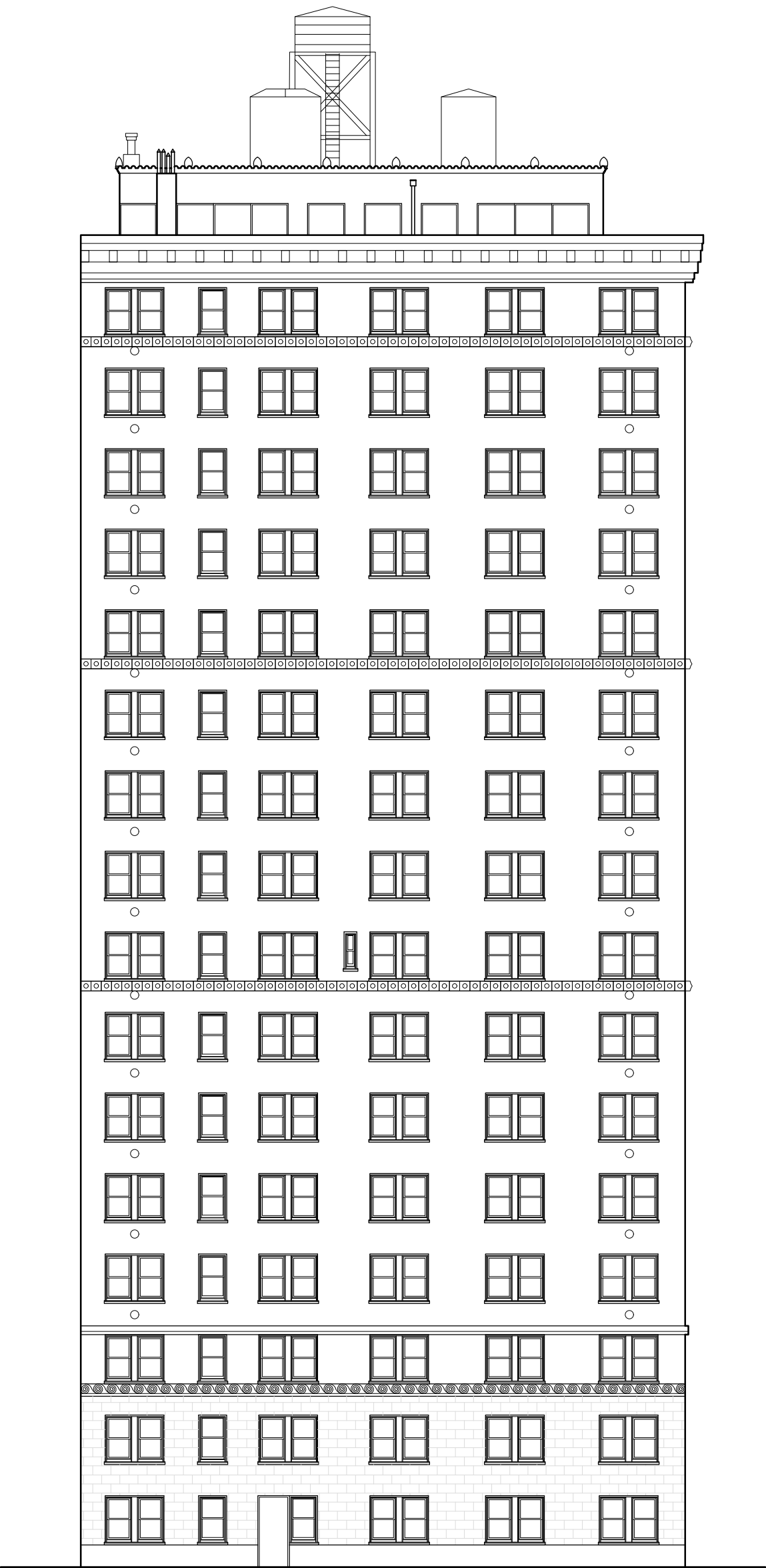
2 East Elevation Proposed 1/16"=1'-0"
