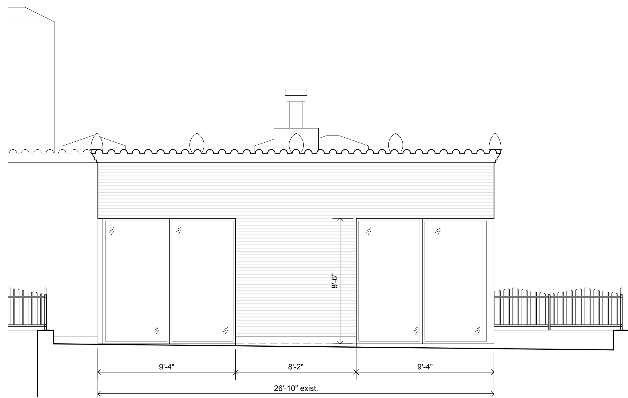
2 South Elevation Proposed 1/4"=1'-0"
