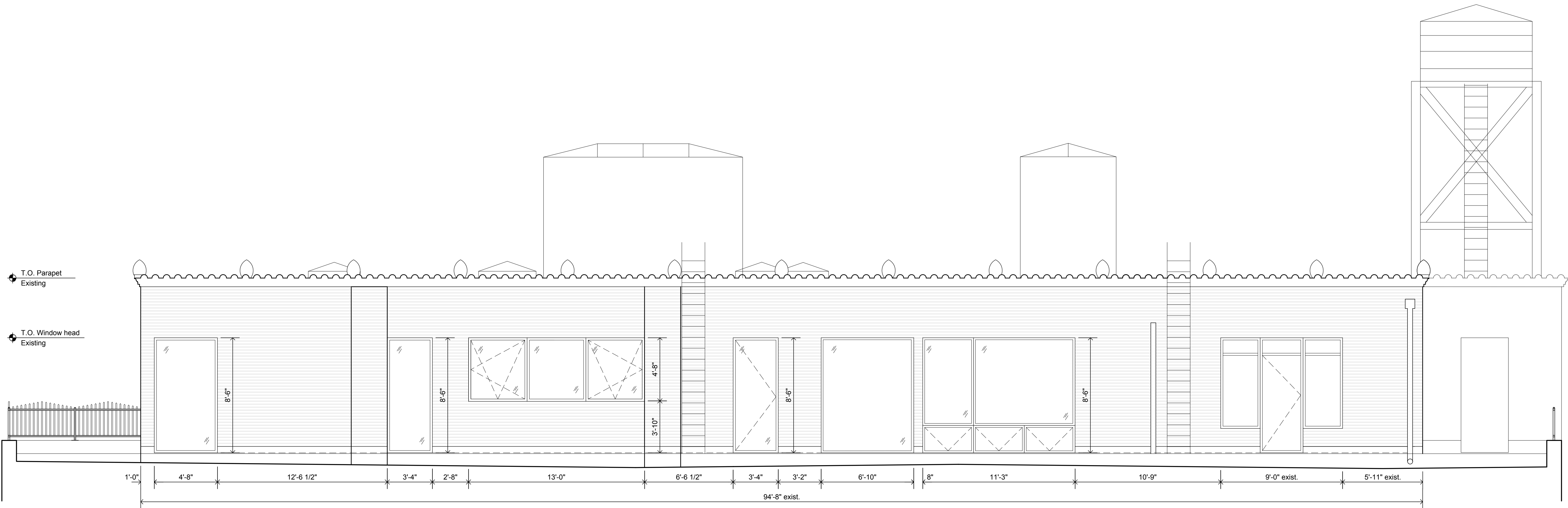
2 North Elevation Proposed 1/4"=1'-0"
