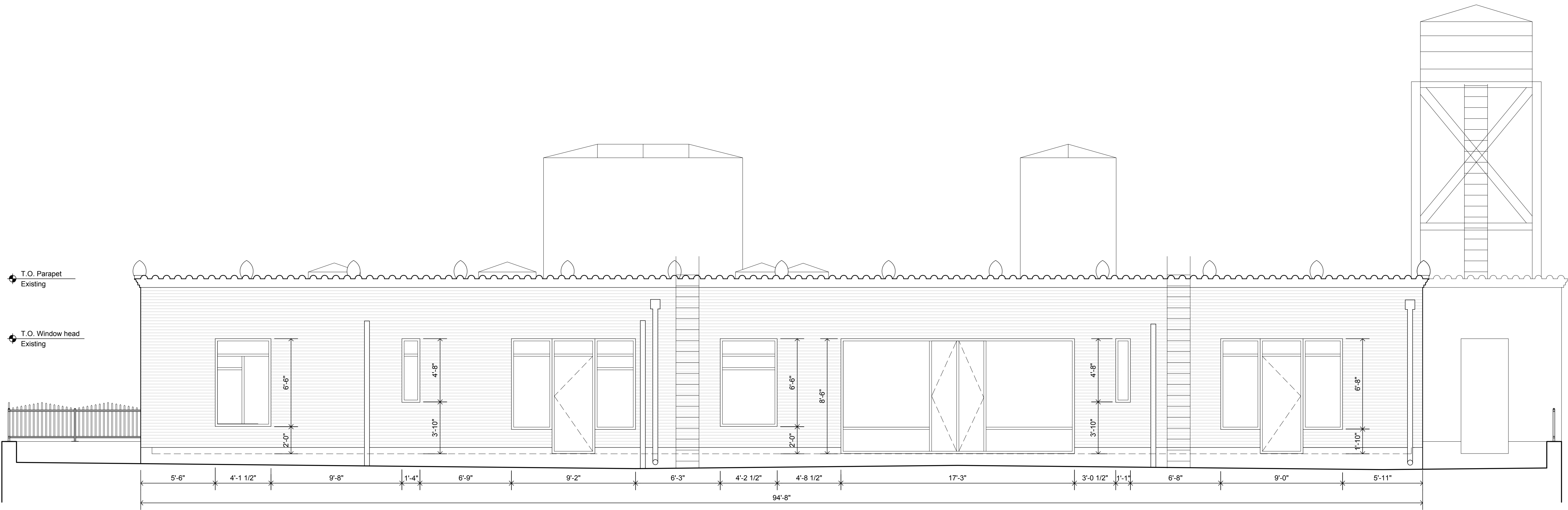
1 North Elevation Existing 1/4"=1'-0"
