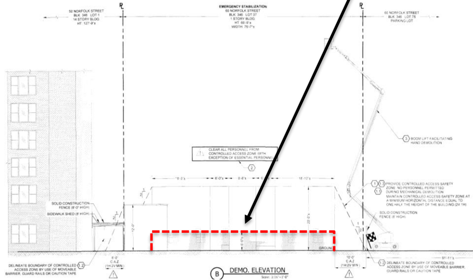
East Elevation
