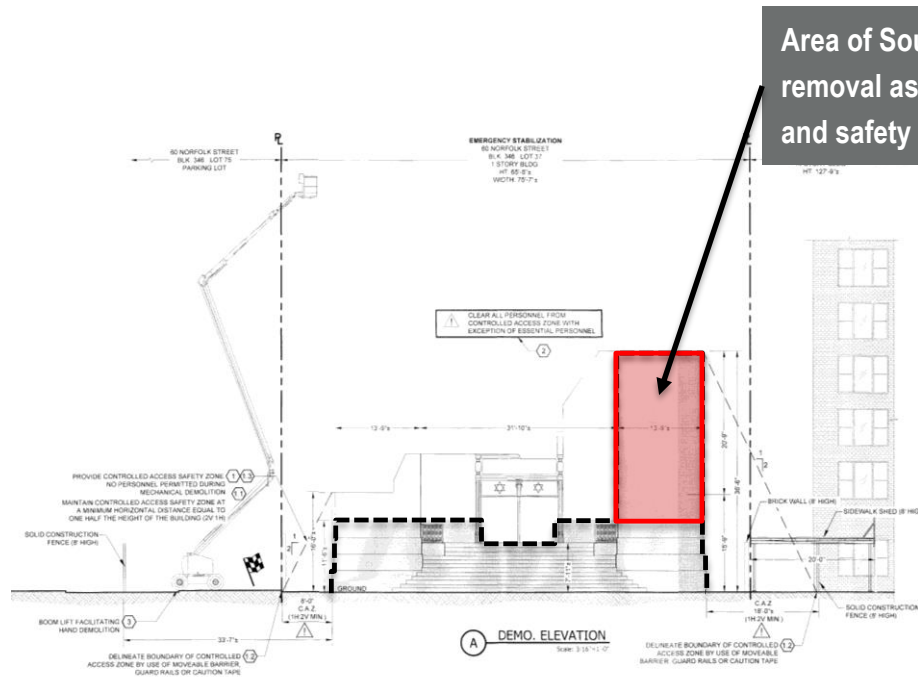
West Elevation
