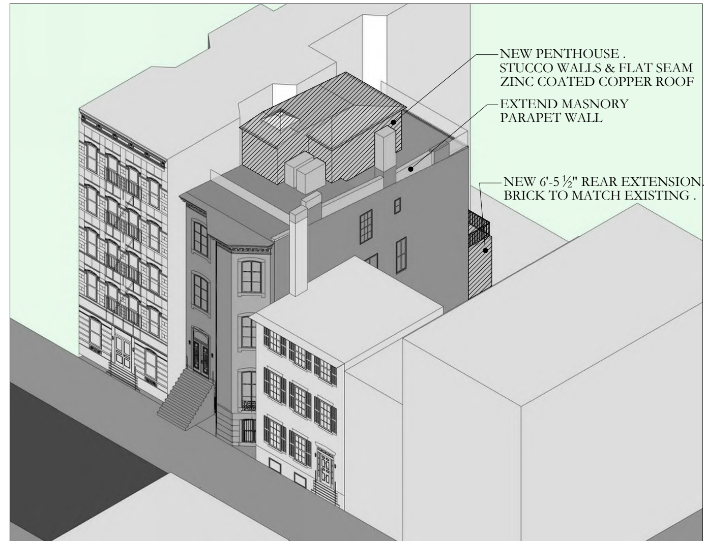
02 LC-11 PROPOSED FRONT AXON DIAGRAM N.T.S.
