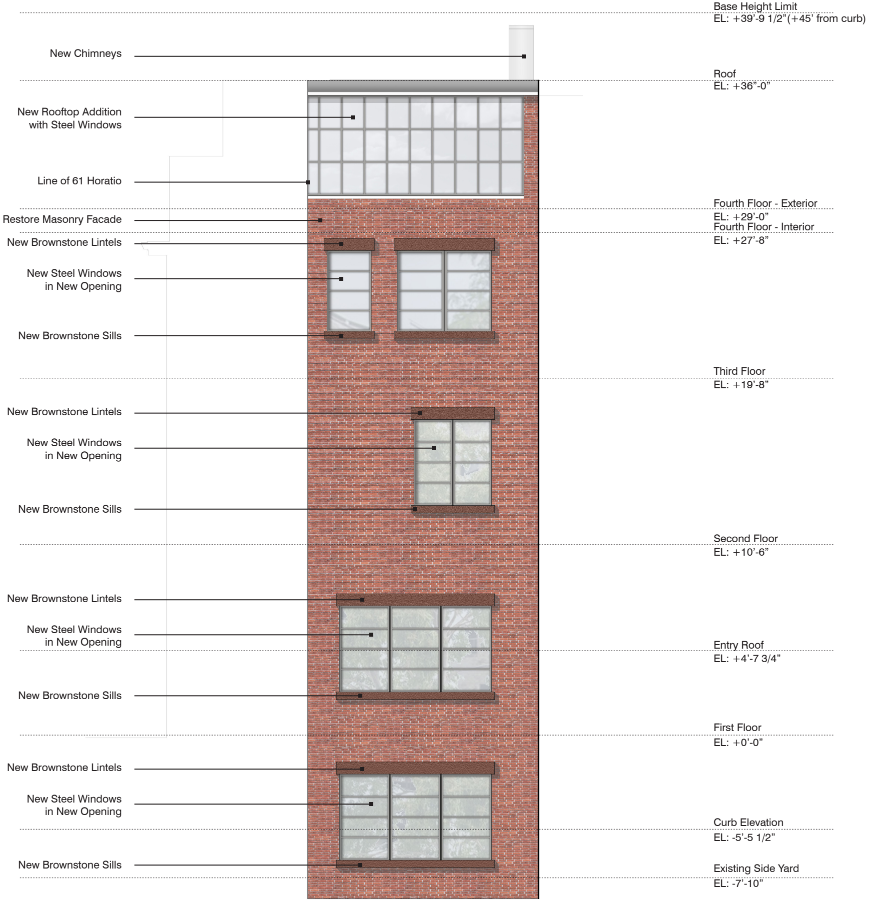
Proposed Elevation
