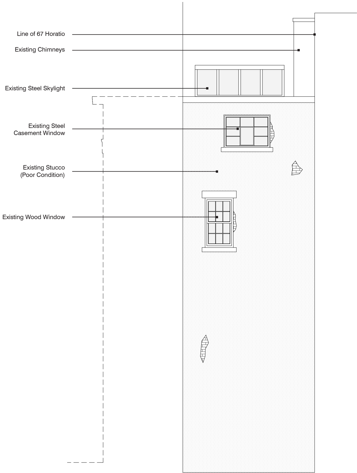
Existing Elevation
