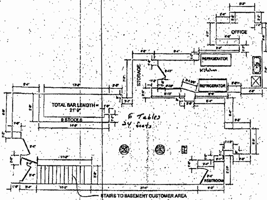
INTERIOR DIAGRAM 1 ST FLOOR 158 E. Houston St September 12, 2007 SCALE: 1" = 3/16"
