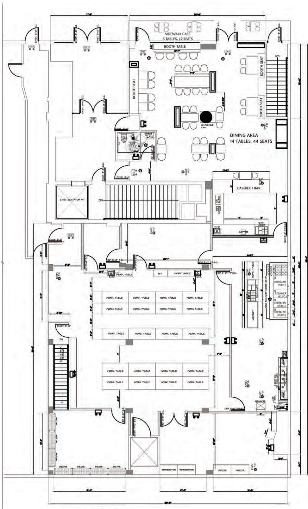
FLOOR PLAN - 1ST FLOOR SCALE: 1/8"=1'-0"
