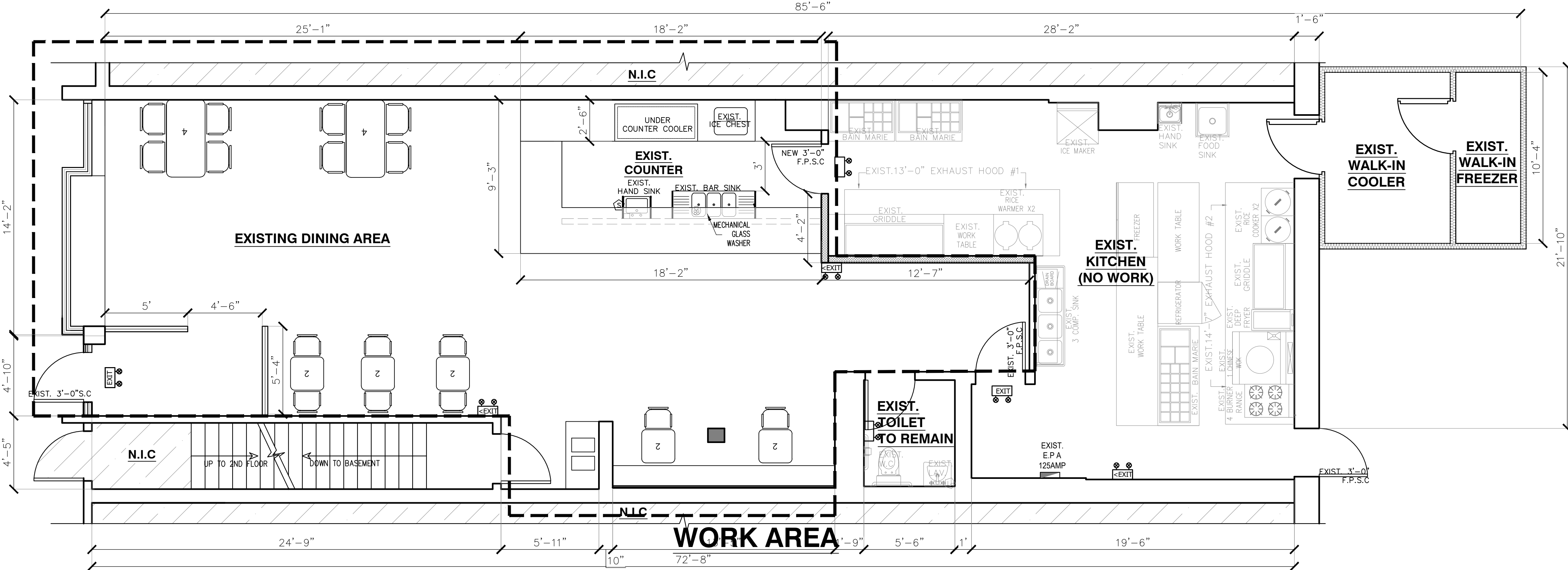
PROPOSED 1ST FLOOR PLAN SCALE: 1/4"=1'-0"
