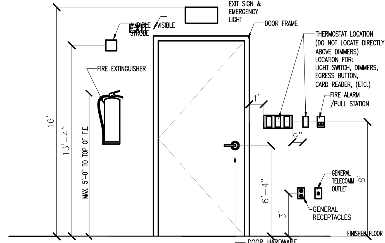
INTERIOR DEVICE MOUNTING HEIGHTS DETAIL SCALE: 1/2"=1'-0" NOTE: ALL DIMENSIONS TO CENTER LINE OF DEVICES.
