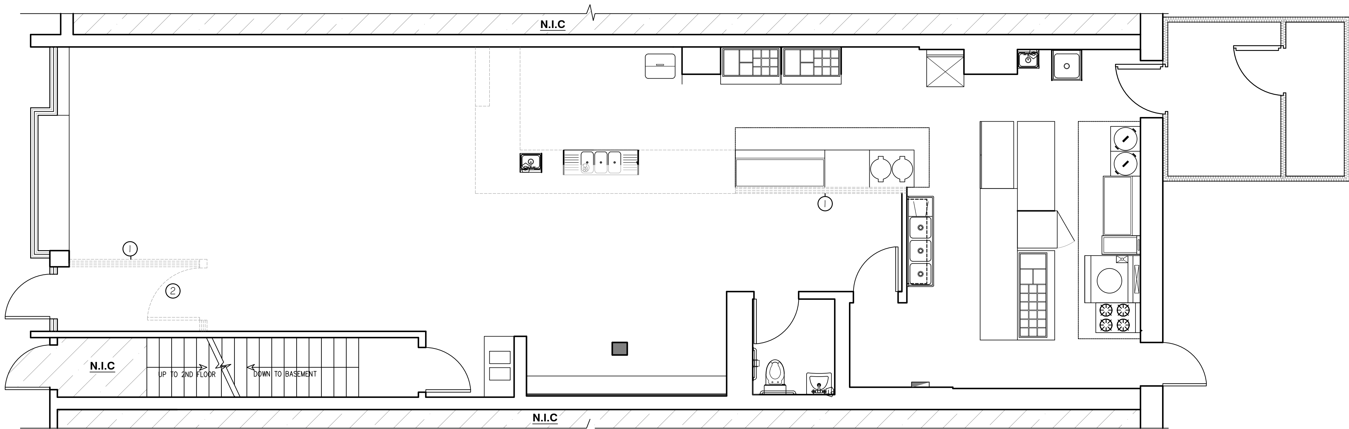
DEMOLITION 1ST FLOOR PLAN SCALE: 1/4"=1'-0"
