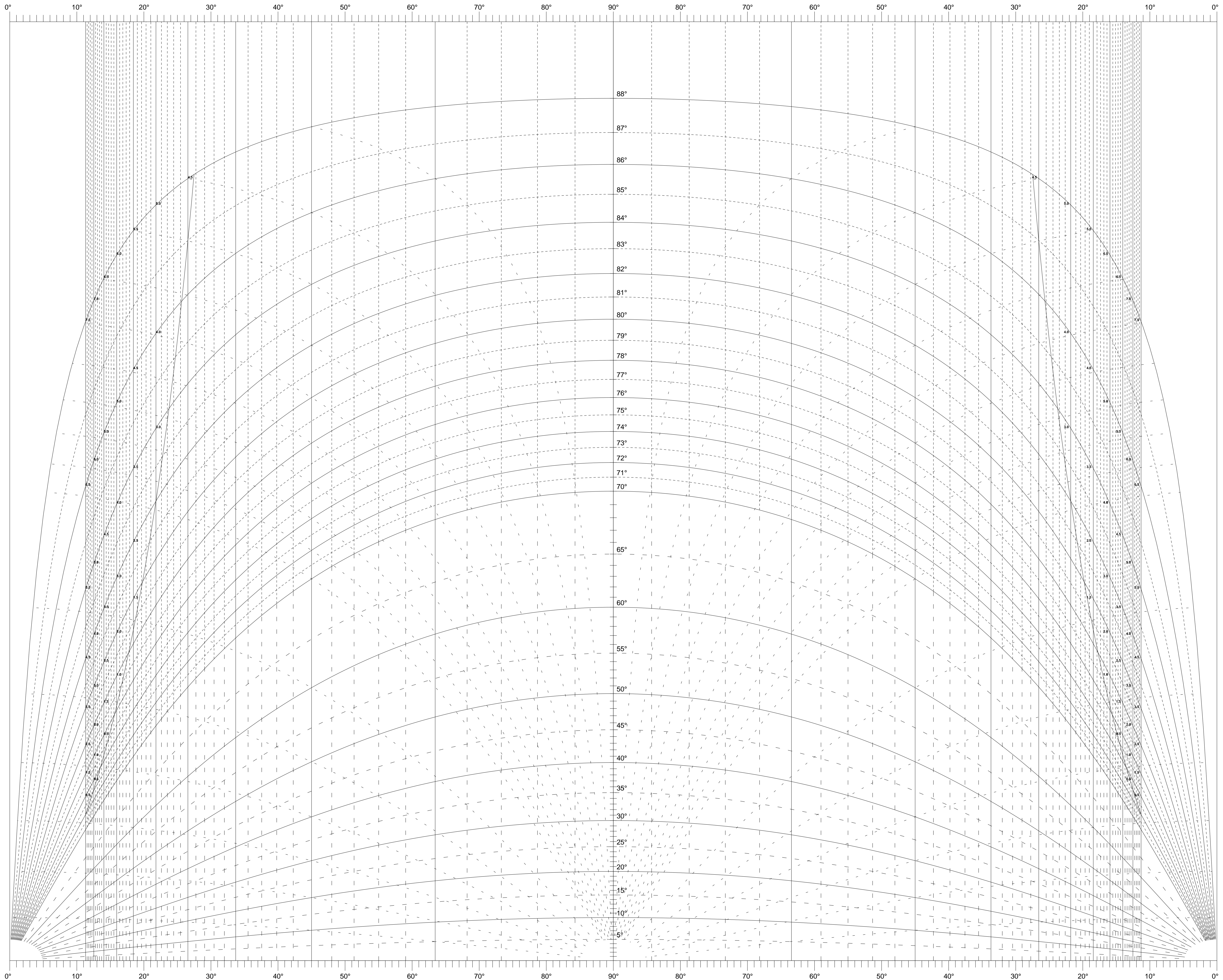
DAYLIGHT EVALUATION DIAGRAM - 100 FOOT STREET
