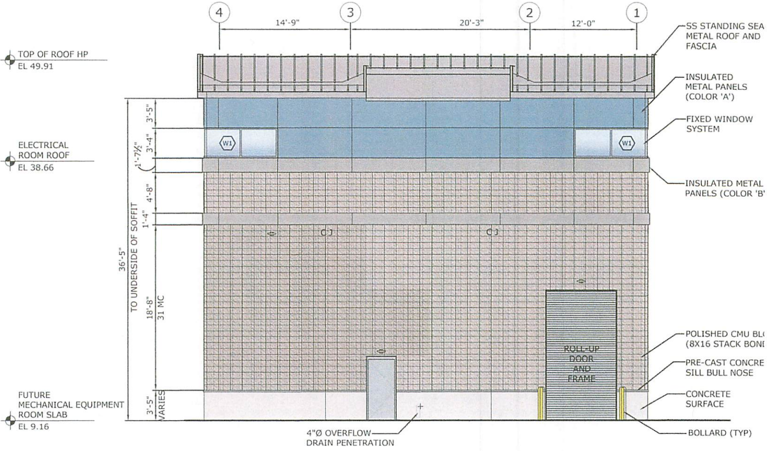
NORTH ELEVATION
