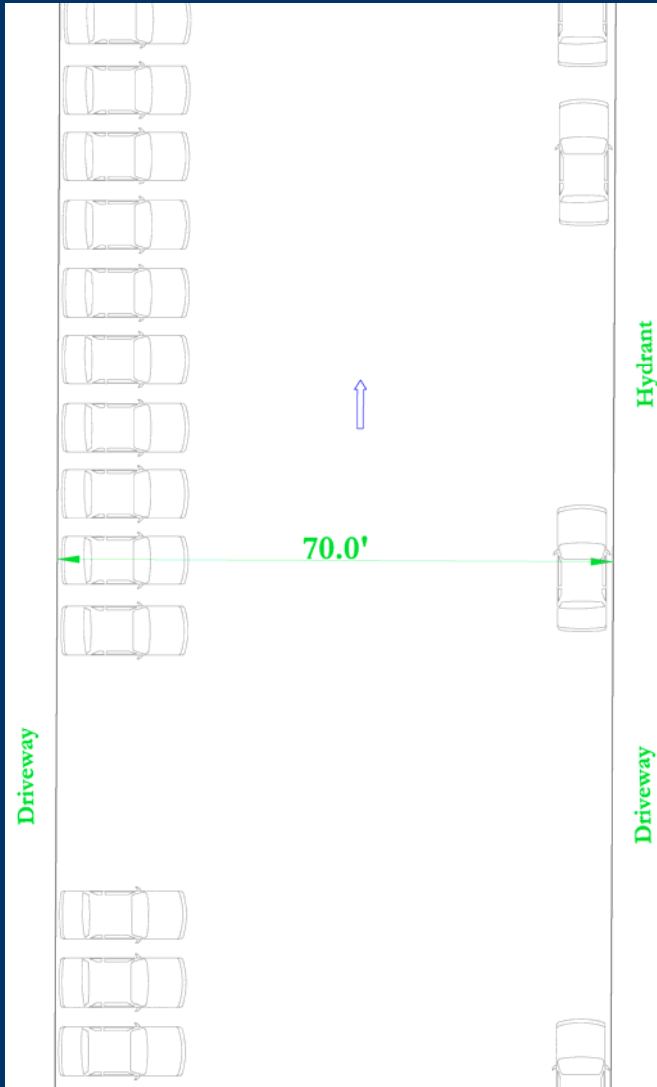
Pre-2007 Angled Parking
