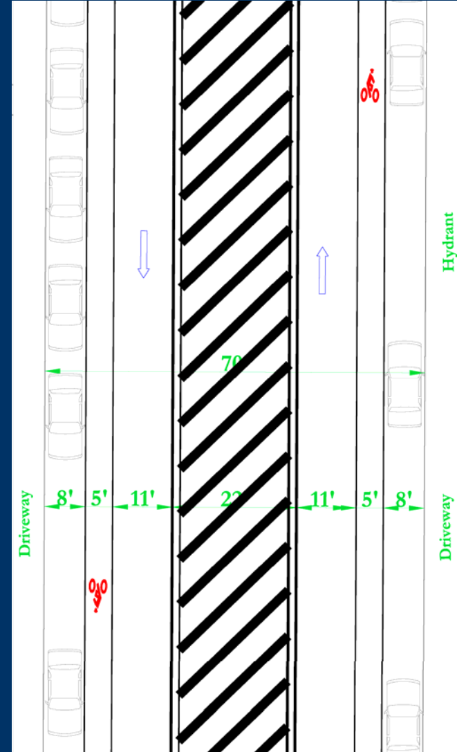
Current Bike Lane
