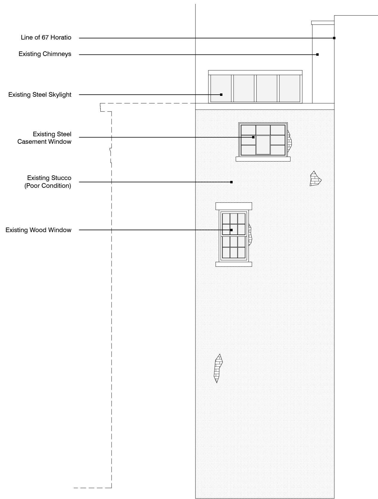
Existing Elevation
