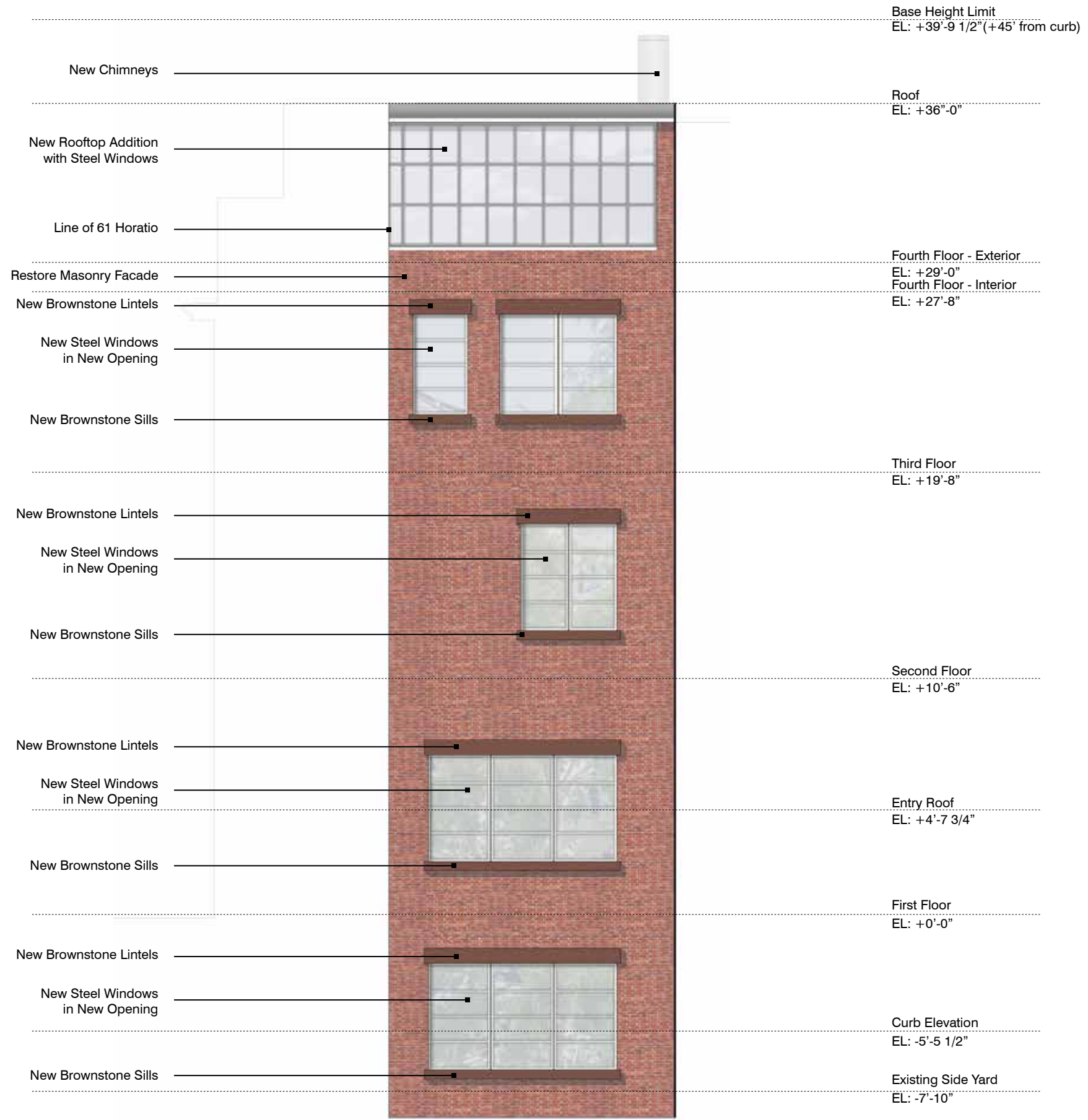
Proposed Elevation
